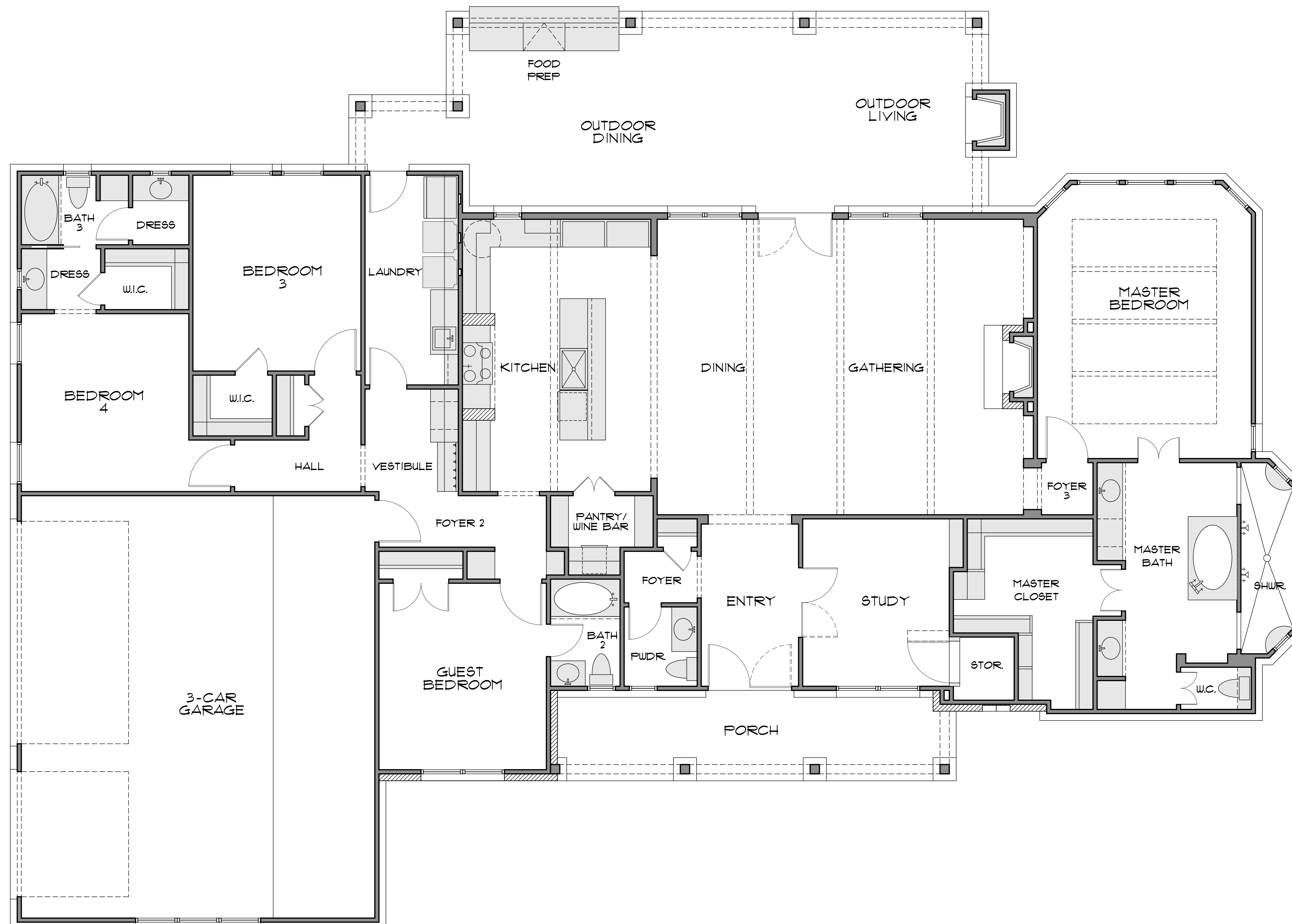
FLOOR PLAN - 2960
